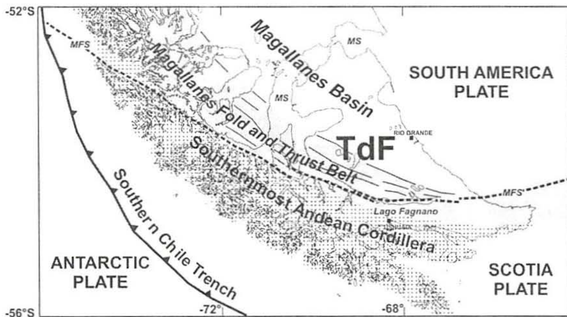
Figure 4. Simplified tectonic map of the southernmost South America and Tierra del Fuego, showing the curved trend of the Magallanes-Fagnano transform system (MFS). TdF: Tierra del Fuego Island; MS: Magallanes Strait
