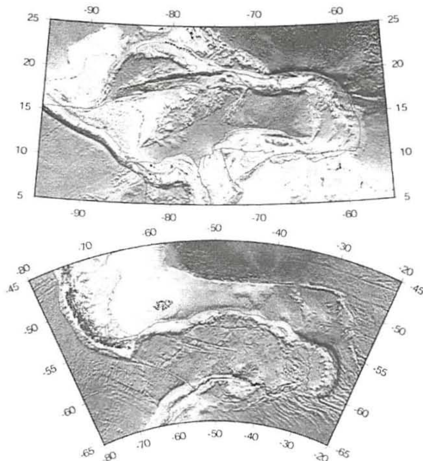
Figure 1. General morphostructural map of the Caribbean (top) and Scotia (bottom) Arcs, with their tectonic boundaries
