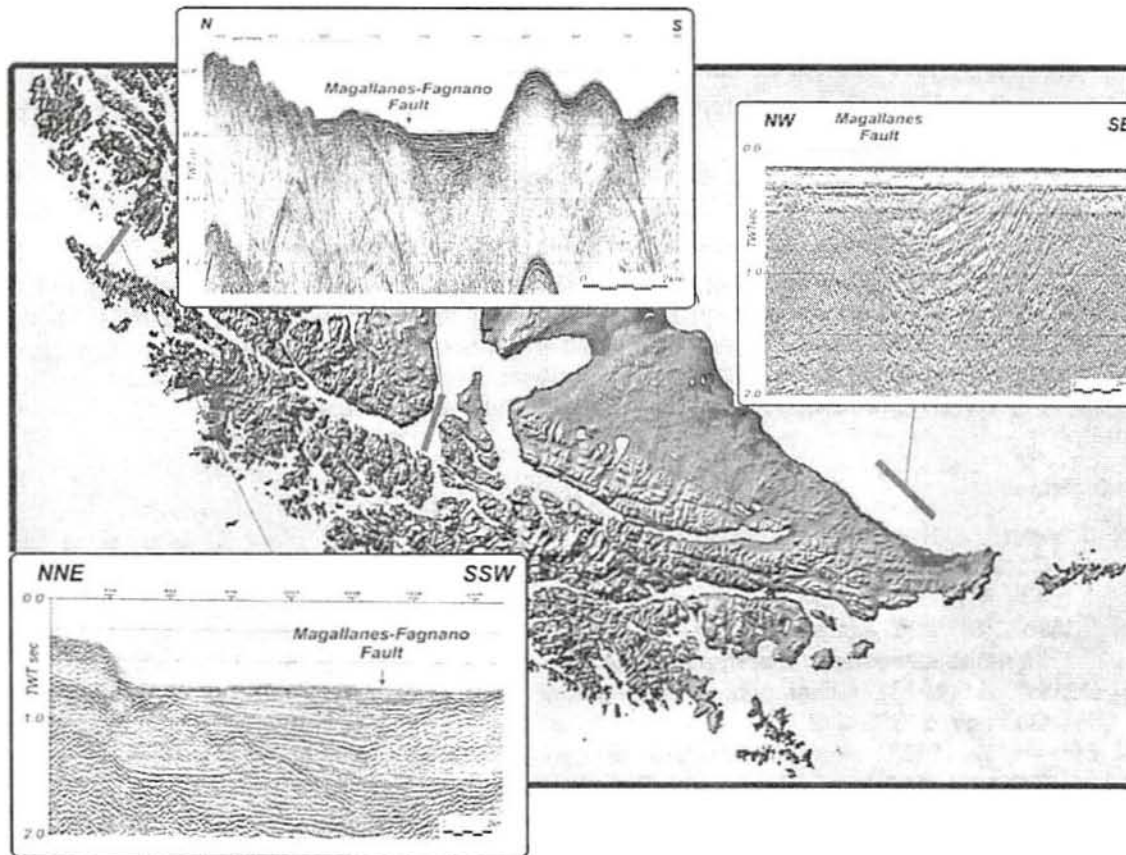
Figure 5. Examples of three seismic profiles acquired across the pull-apart basins formed along the principal deformation zone of the transform system from the Atlantic offshore to the Pacific entrance of the Magallanes Strait (thick segments indicate the location of the profiles). Data show the remarkable asymmetry of the depositional cover of the basins, indicating simultaneous strike-slip motion and transform-normal extension
