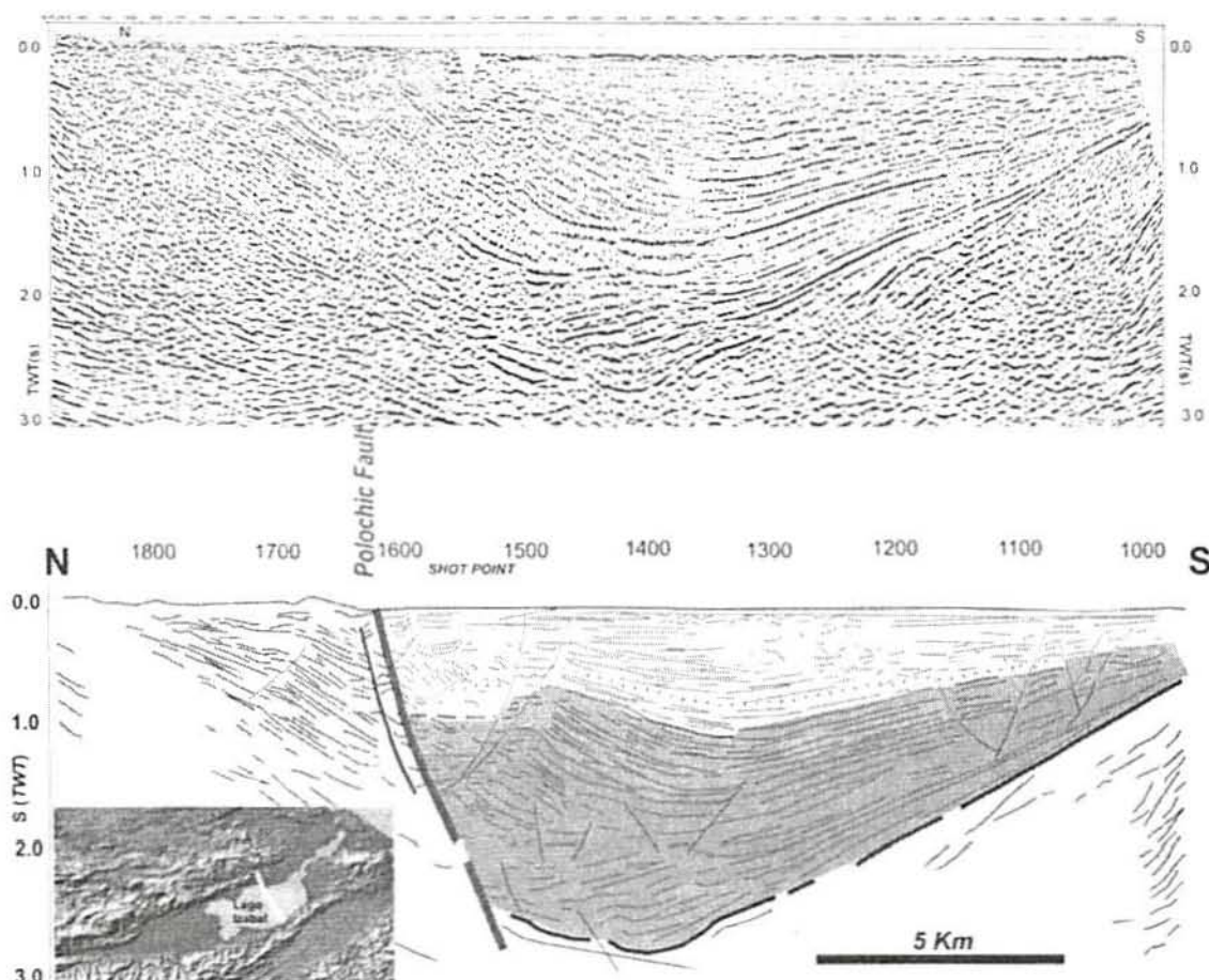
Figure 3. Example of a seismic profile crossing the Lago Izabal, the most important pull-apart basin formed along the transform system, and showing the peculiar asymmetry of the sedimentary cover
