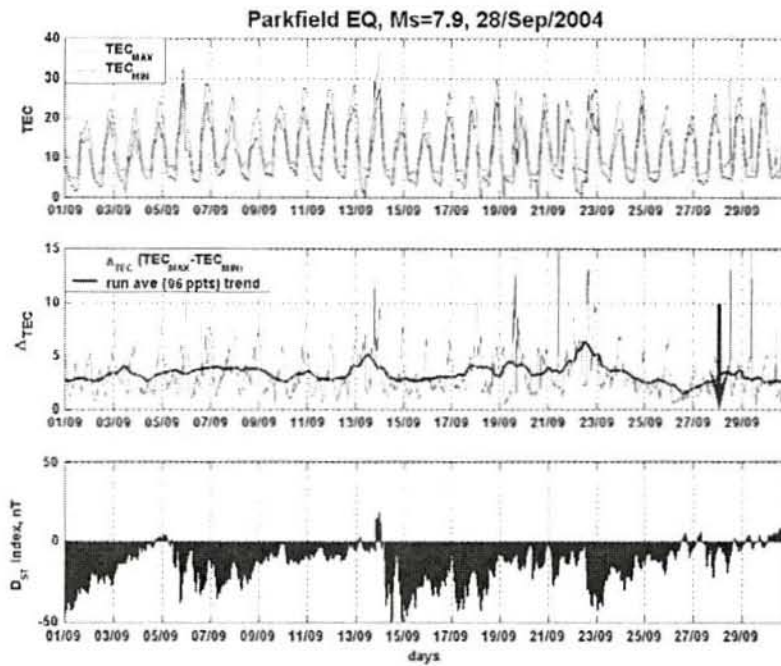
Figure 3. Variation of \Delta_{TEC} = TEC_{max} - TEC_{min} between September 1 and September 29, 2004 at Parkfield. The day of the seismic shock and magnitude of the EQ is indicated in the top of the figure
