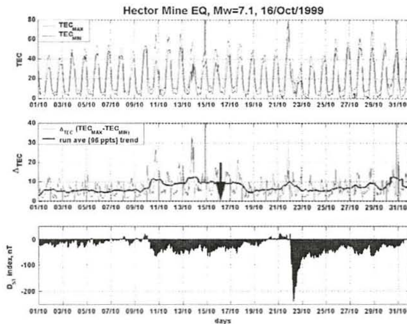
Figure 4. Variation of \Delta_{TEC} = TEC_{max} - TEC_{min} between October 1 and October 31, 1999 at Hector Mine. The day of the seismic shock and magnitude of the EQ is indicated in the top of the figure
