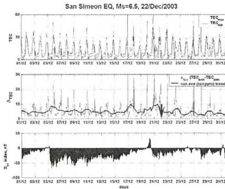
Figure 2. Variation of TEC = TEC_{maxima} - TEC_{minima} between December 1 and December 31, 2003 at San Simeon. The day of the seismic shock and magnitude of the EQ is indicated in the top of the figure
