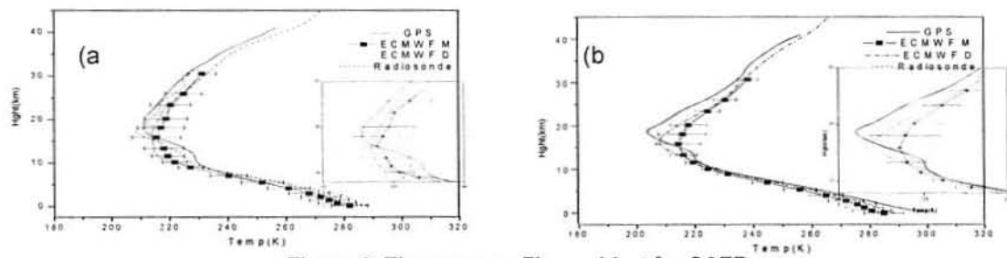
Figure 3. The same as Figure 1 but for SAZR on a) November 29, 2001, CHAMP b) January 22, 2002 CHAMP
