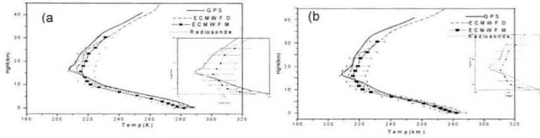
Figure 2. The same as Figure 1 but for SAZR on a) November 24, 2001, SAC-C b) November 26, 2001 CHAMP
